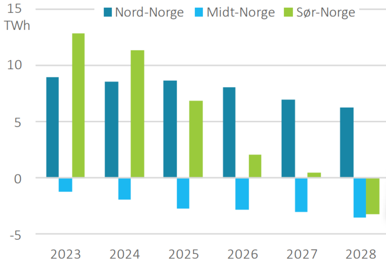
Regional energibalanse i Norge i Basis (TWh)
